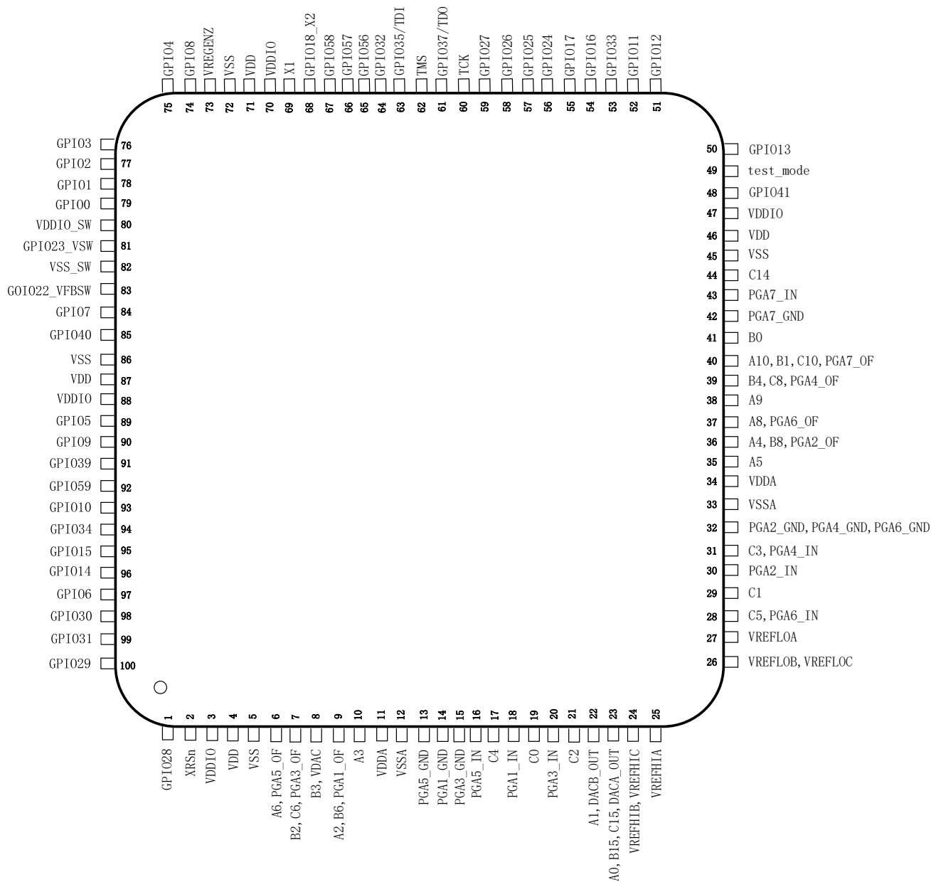
PZP (100-Pin)
